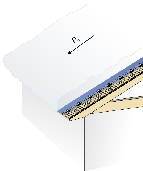
Figure 3. Schematic illustration of snow loads on a roof.
