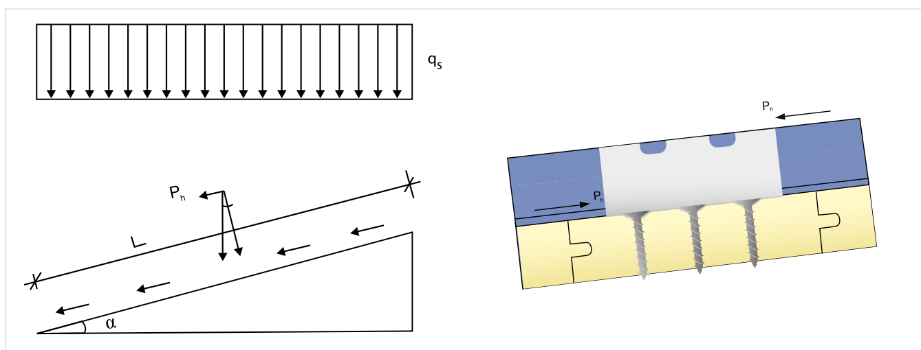
Figure 4. Force transfer via fixed clips to the fixed substrate. Strength values according to technical information.
